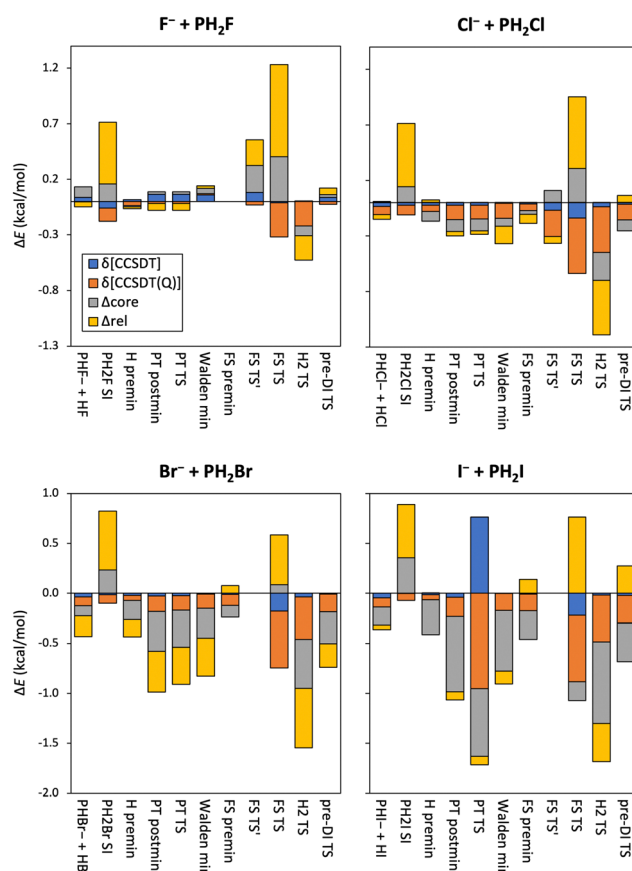
Fig. 3 Post-(T), scalar relativistic and core-correlation corrections to the relative energies of the stationary points of the X^- + PH_2X [ X = F, Cl, Br, I ] identity reactions. \delta[\text{CCSDT}] = \Delta E(\text{CCSDT}/\text{aug-cc-pVDZ}) - \Delta E(\text{CCSD(T)}/\text{aug-cc-pVDZ}) , \delta[\text{CCSDT(Q)}] = \Delta E(\text{CCSDT(Q)}/\text{aug-cc-pVDZ}) - \Delta E(\text{CCSDT}/\text{aug-cc-pVDZ}) , \Delta_{\text{core}} = \Delta E(\text{AE-CCSD(T)}/\text{aug-cc-pwCVTZ}) - \Delta E(\text{FC-CCSD(T)}/\text{aug-cc-pwCVTZ}) , and \Delta_{\text{rel}} = \Delta E(\text{DK-AE-CCSD(T)}/\text{aug-cc-pwCVTZ}) - \Delta E(\text{AE-CCSD(T)}/\text{aug-cc-pwCVTZ}) .
