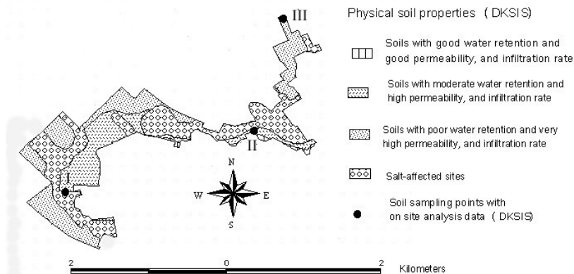
Fig. 1 Physical soil properties in the study area and three soil sampling points with on-site analysis data (based on DKSIS – Pásztor et al. 2002, 2006, Szabó et al. 2005)
